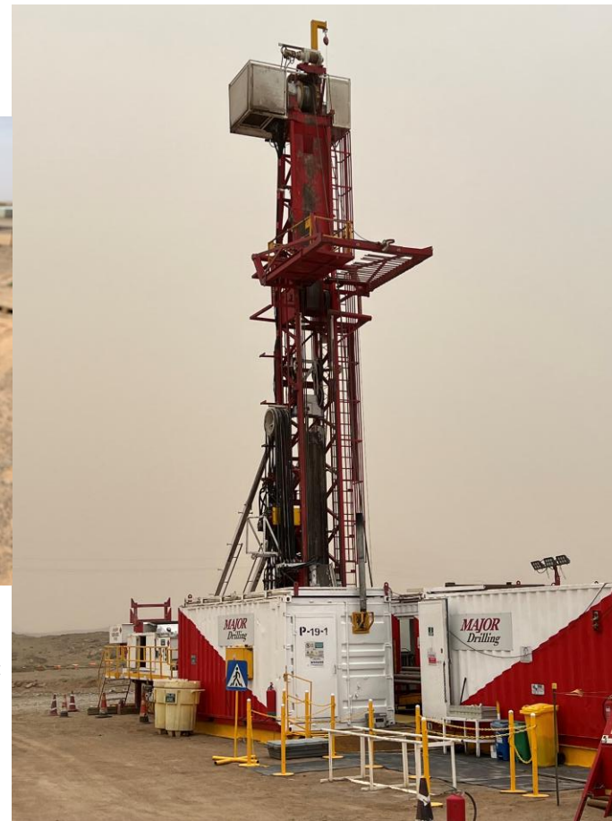
Drill rig at HNE surface hole EGD189. Source: Entrée Resources Ltd. files May 2024.
