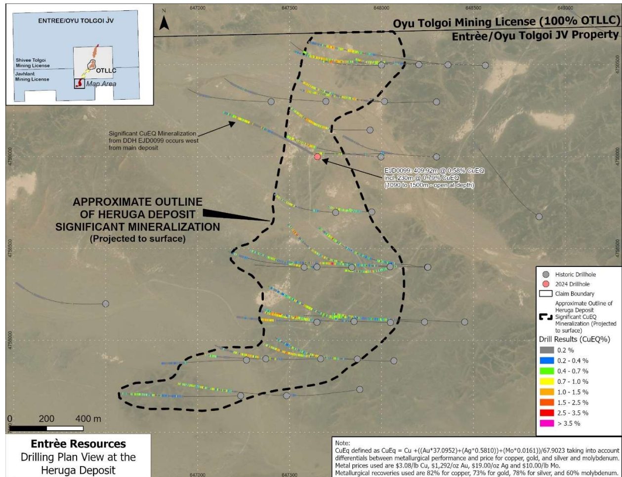
Figure 4: Drilling Plan View of Heruga Deposit
