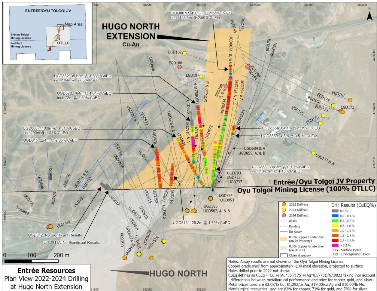
Figure 3: Plan View of Assay Intervals Reported February 27, 2025, and Locations of 2022-2024 Drill Holes
