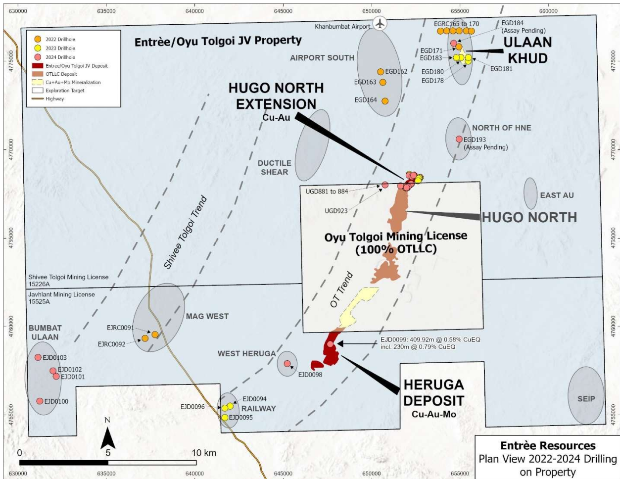
Figure 5: Plan View of 2022 to 2024 Heruga and Regional Drill Holes
